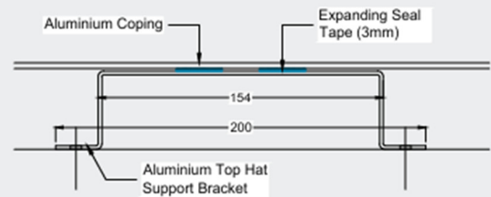
Intermediate Coping Joint Detail
