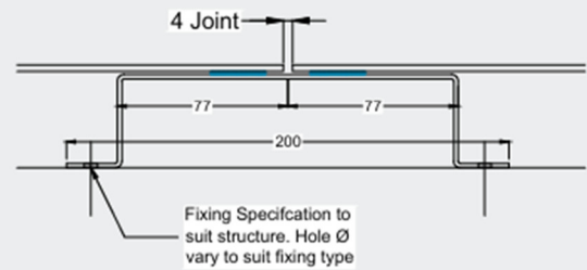
Coping Joint Detail
